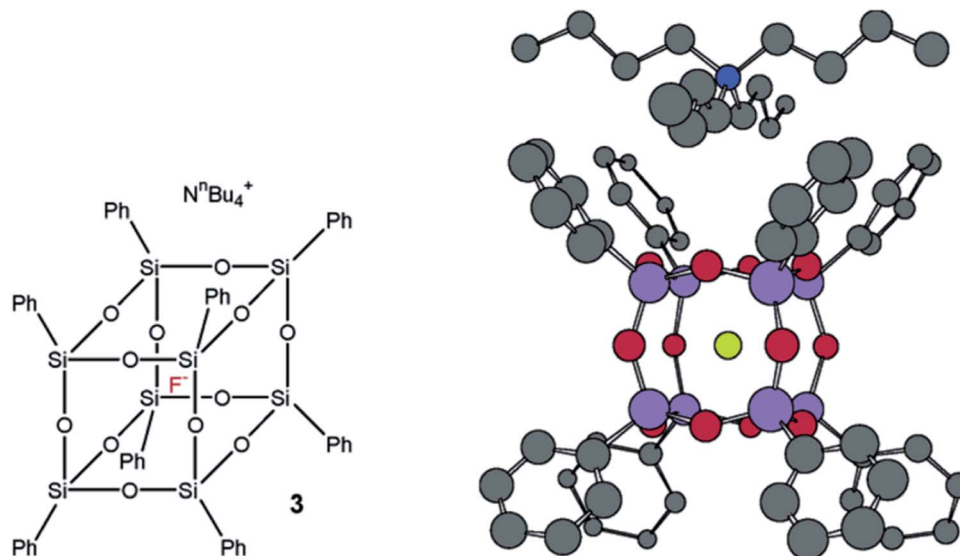
Fig. 10 Octaphenylcubane silsesquioxane with a fluoride anion inside and a tetrabutylammonium counterion outside. Reprinted with permission from ref. 70. Copyright 2020 American Chemical Society.
