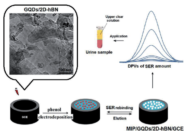
Fig. 9 MIP/GQDs/2D-hBN/GCE process. Reprinted with permission. 148 Copyright 2018, Elsevier.
