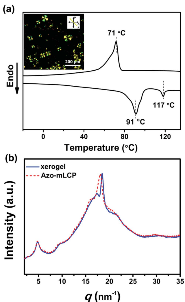
Fig. 7 (a) DSC curves of xerogel tested on the first cooling and second heating scans in \text{N}_2 at a heating rate of 10 ^{\circ}\text{C min}^{-1} . The inset of (a) shows a POM photograph of the xerogel captured at 69 ^{\circ}\text{C} . P, polarizer; A, analyzer; \lambda , phase retarder. (b) 1D WAXD patterns of xerogel and Azo-mLCP.
