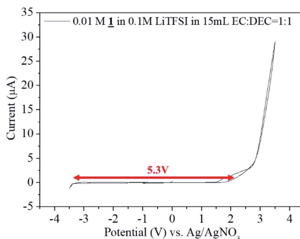
Fig. 7 Cyclic Voltammogram for the sample 1 in 0.1 M LiTFSI in 15 mL EC : DEC = 1 : 1 vs. Ag/AgNO 3 .
