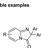
Sierra and co-workers' method 10 examples, 41-85%
