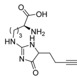
Johannsen and co-workers' method AlkMG-H1 chemical probe One example, 73%
