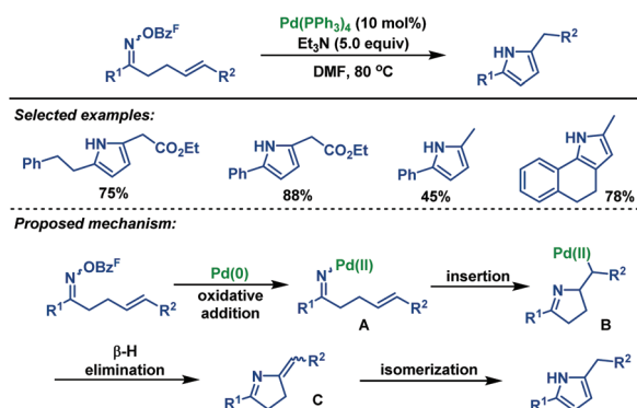
Scheme 32 Narasaka's palladium-catalyzed Heck-type cyclization of \gamma,\delta -unsaturated oxime: synthesis of pyrrole derivatives.
