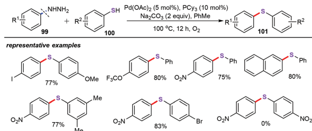
Scheme 37 Palladium-catalyzed oxidative cross-coupling of arylhydrazines with arenethiols.
