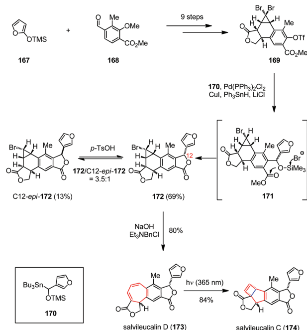
Scheme 24 4π electrocyclic cyclization in the total synthesis of salvileucalin C.
