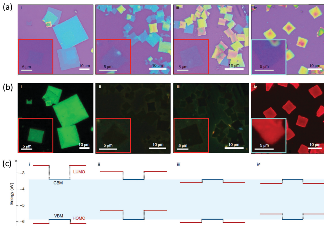
Fig. 6 Optical properties of the hybrid halide perovskites quantum wells. (a) Optical microscopy images of the assembled 2D crystals grown on \text{SiO}_2/\text{Si} substrates: (i) (2\text{T})_2\text{PbI}_4 , (ii) (4\text{Tm})_2\text{PbI}_4 , (iii) (4\text{TCNm})_2\text{PbI}_4 and (iv) (\text{BTm})_2\text{PbI}_4 . The insets are images for monolayer-thick single-quantum-well structures. (b) The corresponding PL images of the assembled 2D crystals under ultraviolet excitation. (c) The corresponding energy level alignments (relative energy levels) of organic (dark red lines) and inorganic (dark blue lines) layers within the hybrid 2D perovskites. Reproduced from ref. 25 with permission from the Springer Nature.
