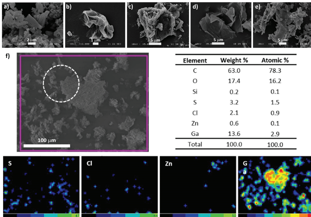
Fig. 5 Scanning Electron Microscopy (SEM): micrographs and corresponding EDX analysis of complexes and nanocomposites. (a) Complex 2 ; (b) GO; (c) 2@GO ; (d) Ga@GO and (e) Ga-2@GO. Scale bars: (a) 2 μm, (b) 1 μm, (c), (d) and (e) 5 μm. (f) SEM image and corresponding EDX elemental analysis and EDX mapping image (S, Cl, Zn, Ga) of Ga-2@GO nanocomposite.
