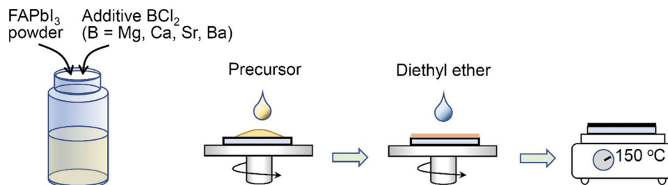
Fig. 1 A schematic illustration of the perovskite deposition procedure. The precursor solution was prepared by mixing the pre-synthesized FAPbI 3 powder with BCl 2 additive (B = Mg, Ca, Sr and Ba), which was spin-coated. Diethyl ether was dripped for 20 s after rotating the substrate. The film was annealed at 150 °C in an air atmosphere.
