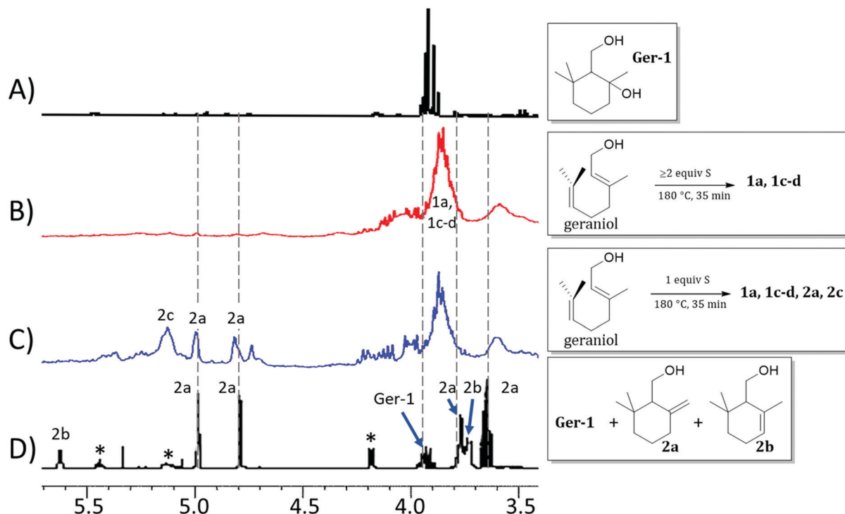
Fig. 2 Proton NMR spectra (CDCl 3 , 300 MHz) for (A) isolated Ger-1 , (B) product mixture resulting from the reaction of geraniol with ≥2 equiv. S, (C) product mixture resulting from the reaction of geraniol with 1 equiv. S, and (D) literature spectrum for a mixture of geraniol (peaks marked with asterisks), 2a and 2b . Spectra (A) and (D) are reprinted from reference 1 ©2005, with permission from John Wiley and Sons.
