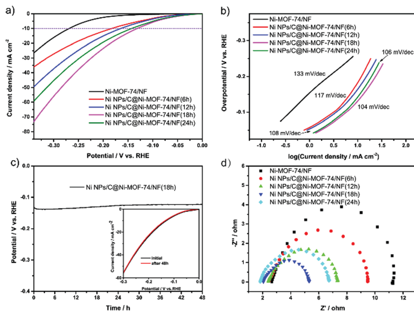
Fig. 4 (a) LSVs of Ni-MOF-74/NF and various Ni NPs/C@Ni-MOF-74/NF measured in 1.0 M KOH at 5.0 mV s -1 without iR compensation; (b) Tafel plots obtained from (a); (c) chronopotentiometric curves of Ni NPs/C@Ni-MOF-74/NF(18 h) at a current density of 10 mA cm -2 ; the inserted image illustrates its LSV curves before and after 48 h; (d) Nyquist plots of various catalysts in 1.0 M KOH solution.
