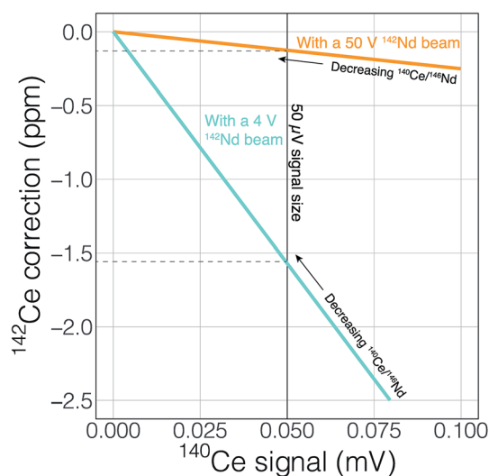
Fig. 10 The magnitude of correction for the isobaric interference of ^{142}\text{Ce} on the ^{142}\text{Nd} measurement as a function of the ^{140}\text{Ce} signal and varying Ce/Nd ratios. Two lines are shown, one with a 50 V ^{142}\text{Nd} beam and the other with a 4 V beam. All calculations were made assuming measurement on a Faraday cup and amplifier equipped with a 10^{11} \Omega resistor. A larger Nd signal will allow for more precise detection and application of important interferences, even if such interferences are not reduced. The same logic and calculations can be applied to many different types of analyses.
