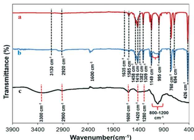
Fig. 8 FTIR analysis of a) ZIF-8, b) ZIF-8-GA, and c) GA.
