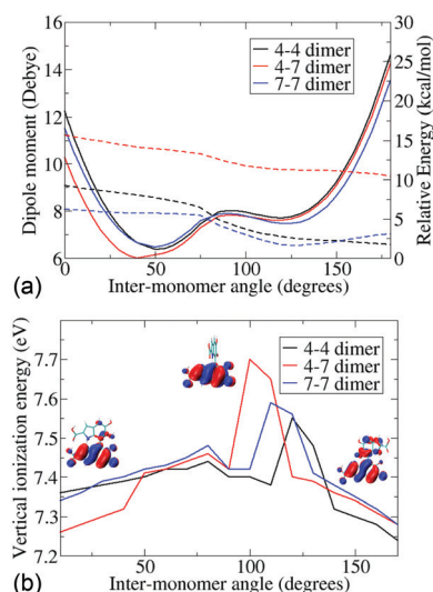
Fig. 2 (a) The relative energies, in kcal mol −1 (marked with solid lines), and dipole moments, in Debye (marked with dashes lines) of the 3 dimers with respect to the inter-monomer angles. (b) The vertical ionization energies (in eV) of the 3 isomers with respect to inter-monomer angles. The orbital from which ionization occurs is shown at 0°, 120° and 170°.
