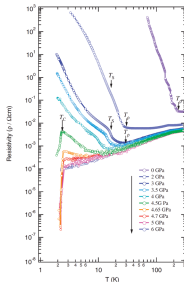
Fig. 16 Temperature dependence of resistivity of (\text{TMTTF})_2\text{AsF}_6 under various pressures, where T_{\beta} , T_s , and T_c are temperatures at minimum resistivity, spin-Peierls transition, and superconducting transition, respectively. Adapted with permission from ref. 72. Copyright 2007 Physical Society of Japan.
