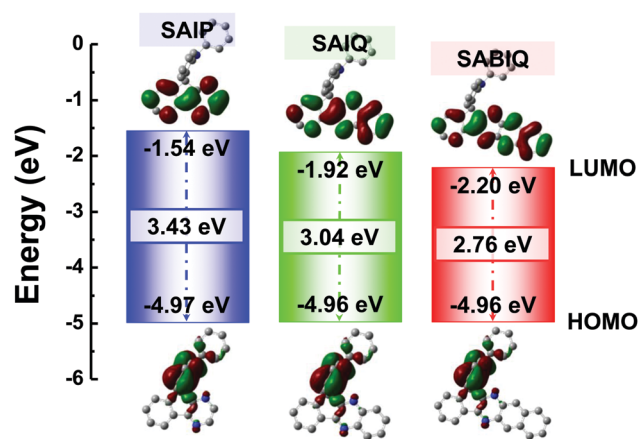
Fig. 7 Frontier molecular orbital distributions and energy levels of SAIP, SAIQ, and SABIQ.
