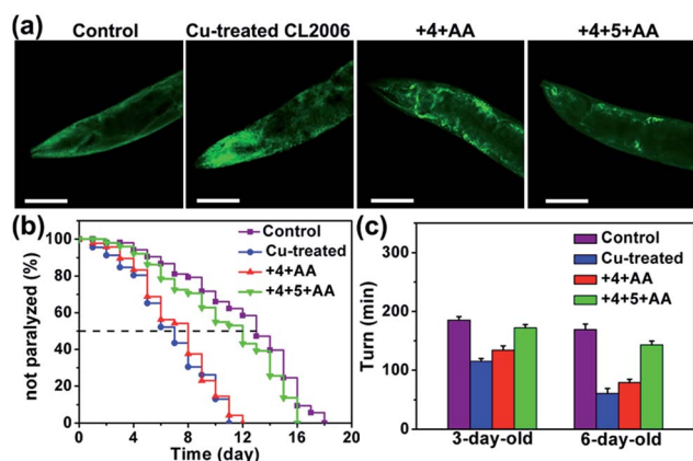
Fig. 5 The in situ synthesis of compound 6 for suppressing the toxicity induced by \text{A}\beta\text{-Cu} fibrils in worms. (a) Representative ThT-staining images of N2 and Cu-treated CL2006 in the presence or absence of prodrug-loaded MSN on the 6th day. Scale bars: 40 \mu\text{m} . (b) Survival curves. (c) Quantification of the worm movement in M9 buffer (turns per minute). Each experiment was repeated three times. Error bars indicate \pm s.d. Cu-treated worms were transferred to NGM containing prodrug-loaded MSN-IgG (1 mg \text{mL}^{-1} ) for 24 h before worms were irradiated with UV light (1 W \text{cm}^{-2} ) for 10 min in 20 min intervals 6 times. A wild-type N2 strain was used as the control.
