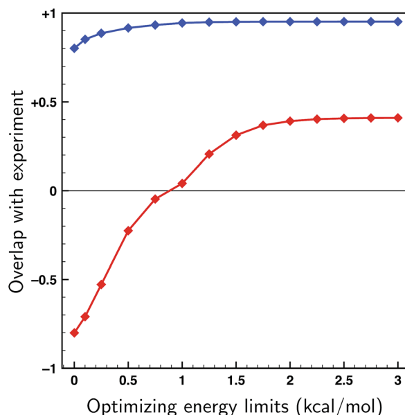
Fig. 6 Fits to the experimental spectra of the two enantiomers of citronellal using the genetic algorithm and the 70 lowest energy conformers of citronellal found within 2 kcal mol −1 at a BP86/TZP level of theory as a function of the maximum energy modulation \Delta E^{\text{max}} . Blue: overlaps from the fit to the correct ( S )-enantiomer. Red: overlaps from the fit to the incorrect ( R )-enantiomer.
