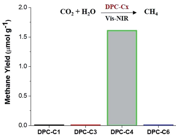
Fig. 11 Photocatalytic \text{CO}_2 conversion to methane using DPC-C1, DPC-C3, DPC-C4, and DPC-C6 as catalysts under light (400 to 1100 nm). No conversion in the dark or in the absence of \text{CO}_2 . Micro-GC with TCD sensitivity >10 ppm. Error in methane yield for DPC-C4: \pm 0.51 .
