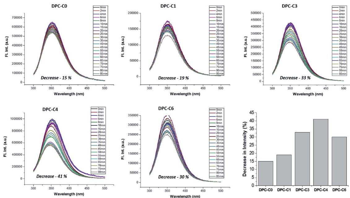
Fig. 12 Steady-state fluorescence of 3.5 mL BSA solution (10 \mu\text{M} prepared in PBS buffer of 0.1 mM) in the presence of DPC-C0, DPC-C1, DPC-C3 and DPC-C6 in light (400 to 1100 nm). Excited at 280 nm and emission recorded from 300–500 nm.
