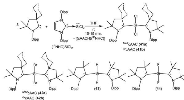
Fig. 11 cAAC coordinated SiR 2 (R = Cl, Br, H, F) dis- and biradicals.
