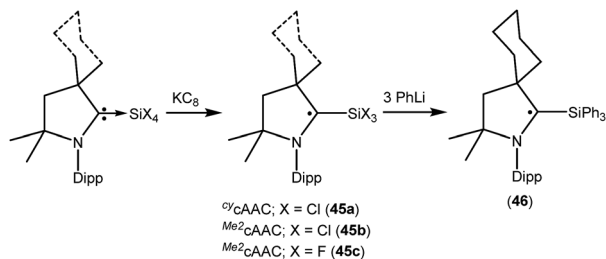
Fig. 12 Synthesis of (\text{cAAC})\text{SiR}_3 (R = Cl, F or Ph).
