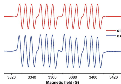
Fig. 19 EPR spectrum of radical anion [(^{\text{Cy}}\text{cAAC})\text{Si}(\text{P-Tip})]_2^\cdot ( 64 •- ) in toluene at 285 K.
