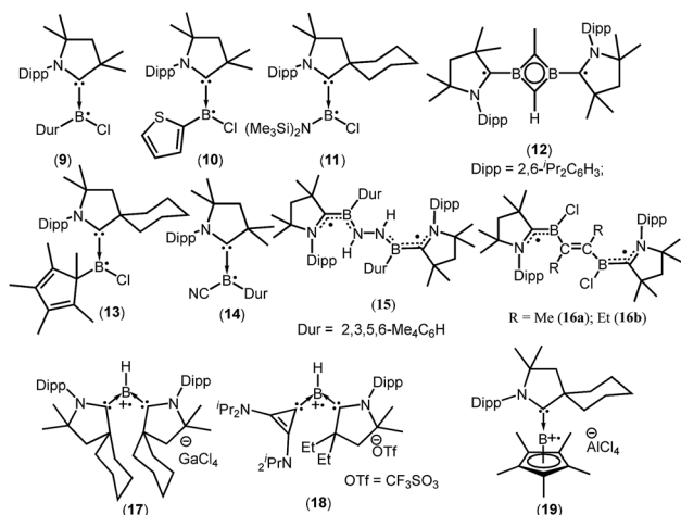
Fig. 2 cAAC ligated boron mono- and biradicals.
