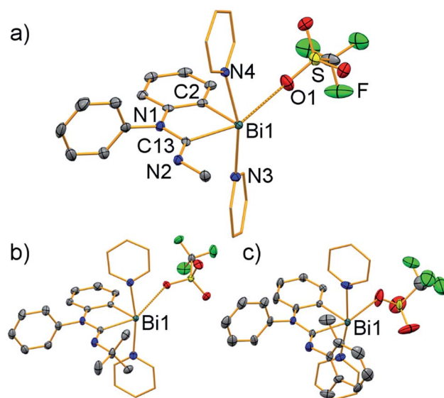
Fig. 4 Molecular structures of [\text{Bi}(\text{CNRNPh}(\text{C}_6\text{H}_4))(\text{NC}_5\text{H}_5)_2][\text{OTf}] in the solid state ((a) 3 (R = Me); (b) 4 (R = t Bu); (c) 5 (R = 2,6- \text{Me}_2\text{-C}_6\text{H}_3 )). Displacement ellipsoids are shown at the 50% probability level; carbon atoms of pyridine ligands are shown as wireframe for clarity. Hydrogen atoms, lattice-bound solvent molecules, and split positions of disordered groups in (c) are omitted for clarity. Atom labelling in (b) and (c) is in analogy with that in (a). Selected bond lengths (Å) and angles ( ^\circ ): (a) Bi1–C2, 2.222(3); Bi1–C13, 2.305(3); Bi1–N3, 2.499(2); Bi1–N4, 2.482(2); Bi1...O1, 3.025(2); C13–N1, 1.402(3); C13–N2, 1.263(3); C2–Bi1–C13, 76.84(10); C2–Bi1–N3, 84.48(8); C2–Bi1...O1, 79.86(9); N3–Bi1–N4, 164.35(7); C13–Bi1...O1, 155.56(8); \tau_5 = 0.15 . (b) Bi1–C2, 2.225(3); Bi1–C13, 2.331(3); Bi1–N3, 2.485(3); Bi1–N4, 2.525(3); Bi1...O1, 2.997(2); C13–N1, 1.415(4); C13–N2, 1.261(4); C2–Bi1–C13, 77.35(12); C2–Bi1–N3, 87.63(11); C2–Bi1...O1, 80.94(10); N3–Bi1–N4, 169.39(9); C13–Bi1...O1, 153.18(9); \tau_5 = 0.27 . (c) Bi1–C2, 2.202(4); Bi1–C13, 2.299(4); Bi1–N3, 2.510(4); Bi1–N4, 2.488(4); Bi1...O1, 2.907(15); C13–N1, 1.43(2); C13–N2, 1.269(6); C2–Bi1–C13, 76.89(15); C2–Bi1–N3, 84.96(14); C2–Bi1...O1, 82.0(3); N3–Bi1–N4, 169.41(13); C13–Bi1...O1, 158.8(3); \tau_5 = 0.18 .
