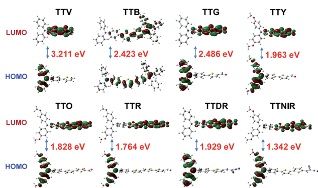
Fig. 4 Molecular orbital amplitude plots of HOMO and LUMO energy levels of TTV, TTB, TTG, TTY, TTO, TTR, TTDR and TTNIR calculated at the B3LYP/6-31+G(d) level based on the geometries optimized at the TD-B3LYP/6-31+G(d) level.
