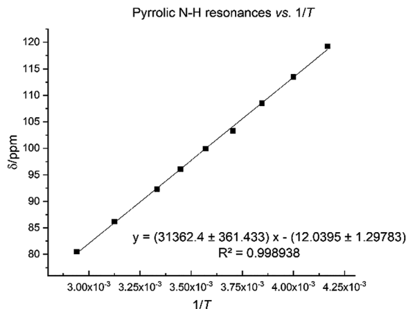
Fig. 7 Temperature dependence of pyrrole 1 H NMR spectroscopic resonance in 8 between 240 K and 340 K.
