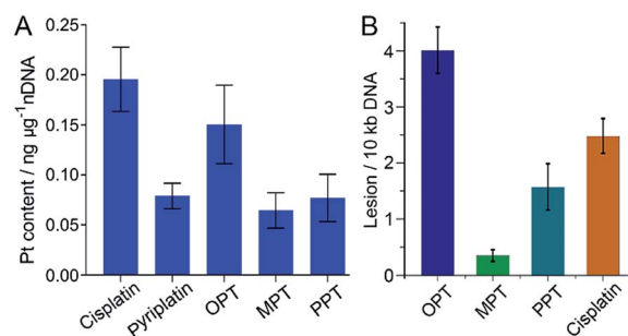
Fig. 3 Content of nDNA-bound Pt in A549 cells after incubation with OPT, MPT, PPT, pyriplatin and cisplatin (10 \mu M), respectively, for 24 h (A), and damage to the D-loop region of mtDNA in A549 cells caused by OPT, MPT, PPT and cisplatin, respectively (B). Data are expressed as mean \pm S.D. of at least three independent experiments.
