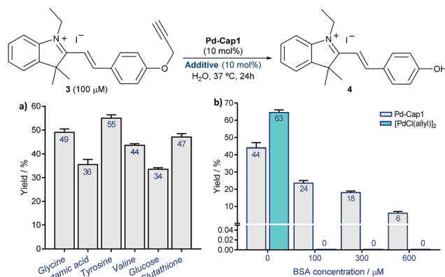
Fig. 4 Pd-Cap1-promoted depropargylation of 3 (mean \pm s.e.m., n = 2 ) in the presence of different additives, 1.0 equiv. with respect to Pd (a), and of increasing concentrations of BSA (b). The reaction is also effective in the presence of higher amounts of the additives as indicated in (a) (see Fig. S12).†
