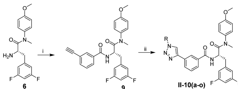
Scheme 2 Reagents and conditions used to synthesize II-10(a-o) . (i) 3-ethynylbenzoic acid, HATU, DIEA, \text{CH}_2\text{Cl}_2 , r.t., 10 h; (ii): azide substituents; \text{CuSO}_4 \cdot 5\text{H}_2\text{O} , VcNa, \text{THF}/\text{H}_2\text{O} ( v : v = 1 : 1 ), 30–60 °C, 4–6 h.
