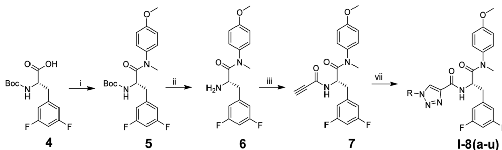
Scheme 1 Reagents and conditions used to synthesize I-8(a-u) . (i) 4-methoxy- N -methylaniline, PyBop, DIEA, \text{CH}_2\text{Cl}_2 , r.t., 8–10 h; (ii): \text{CF}_3\text{-COOH} ; \text{CH}_2\text{Cl}_2 , r.t., 5–6 h; (iii) propiolic acid, HATU, DIEA, \text{CH}_2\text{Cl}_2 , r.t., 10 h; (vii): azide substituents; \text{CuSO}_4 \cdot 5\text{H}_2\text{O} , VcNa, \text{THF}/\text{H}_2\text{O} ( v : v = 1 : 1 ), 30–60 °C, 4–6 h.
