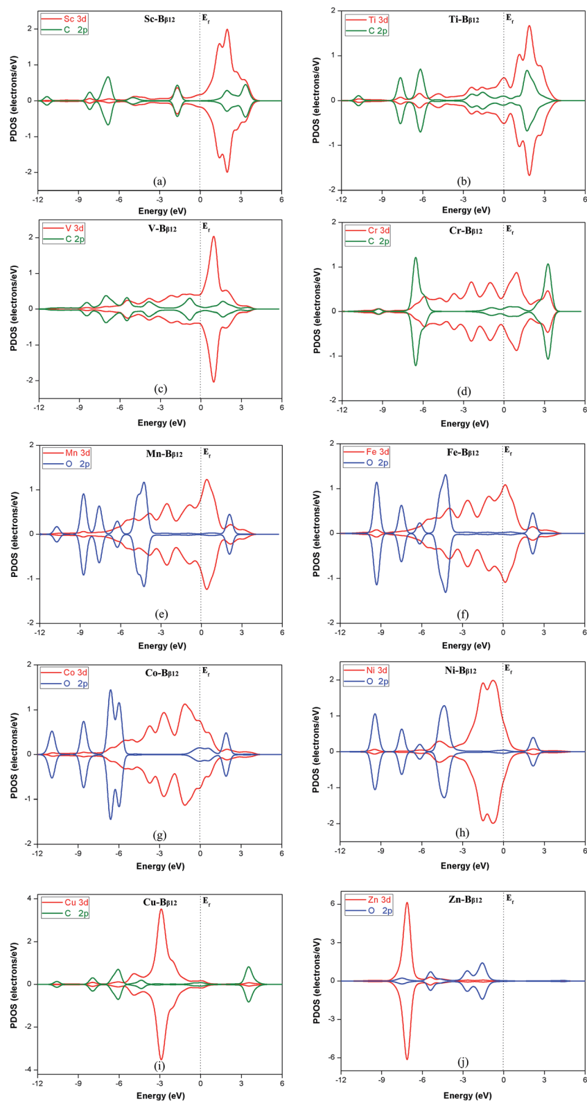
Fig. 6 Projected partial density of states (PDOS) of (a) C*OOH adsorbed on Sc-B p12 , (b) C*HO on Ti-B p12 , (c) C*HOH on V-B p12 , (d) C*O on Cr-B p12 , (e) O*CHOH on Mn-B p12 , (f) O*CHOH on Fe-B p12 , (g) O*H on Co-B p12 , (h) O*CHOH on Ni-B p12 , (i) C*O on Cu-B p12 (j) O*H on Zn-B p12 . The dotted line denotes the Fermi level. The red, blue and green lines represent the 3d orbital of the metal atom, and the 2p orbital of the oxygen and carbon atom, respectively.
