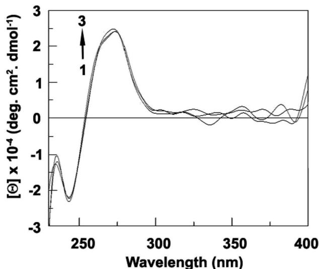
Fig. 15 Intrinsic CD spectra of CT DNA (60 \mu M) in the presence of 0, 6, 12, 18, and 30 \mu M of compound 2.
