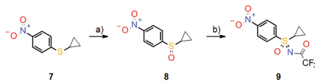
Scheme 4 Synthesis of key sulfoximine building block 9 by rhodium-catalyzed imination of sulfoxide 8 . Reagents and conditions: (a) H_2IO_6 , FeCl_3 , MeCN, rt, 76%; (b) CF_3C(O)NH_2 , PhI(OAc)_2 , MgO, [Rh_2(OAc)_4] , DCM, rt, 78%.
