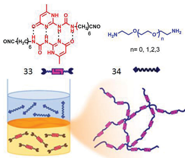
Fig. 16 (top) Structure of the supra-monomer. (bottom) Schematic presentation of interfacial polymerization. Adapted with permission from ref. 56. Copyright 2018, American Chemical Society.
