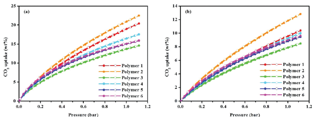
Fig. 4 (a) Volumetric CO 2 adsorption isotherms and desorption isotherms up to 1.13 bar at 273.15 K, and (b) volumetric CO 2 adsorption isotherms and desorption isotherms up to 1.13 bar at 298.15 K.
