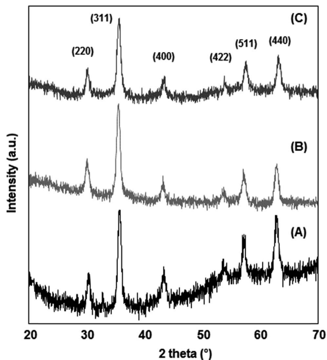
Fig. 2 XRD pattern showing the characteristic magnetite/maghemite diffraction peaks of the prepared nanoparticles: (A) \text{Fe}_3\text{O}_4 ; (B) \text{Fe}_3\text{O}_4@\text{CMC} ; (C) \text{Si}-\text{Fe}_3\text{O}_4@\text{CMC} .
