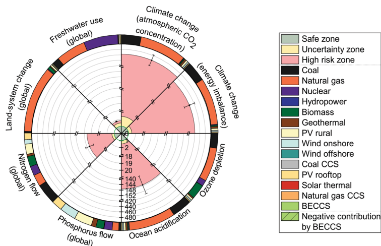
Fig. 3 Global US electricity generation and imports portfolio and performance relative to downscaled planetary boundaries for the Paris Agreement mix (solution S2). The circle on the left represents the energy mix in 2030 that meets the Paris Agreement 2 degrees Celsius target at minimum cost; its performance in terms of planetary boundaries is summarized in a rose chart on the right. The rose chart represents the current performance of each Earth-system process divided by the US power sector share of the full safe operating space (i.e., a value less than one implies it lies below the planetary boundary). The green zone is the safe operating space (i.e., within the strictest planetary boundary in the uncertainty range), the yellow zone is the uncertainty range of each planetary boundary and the red zone is beyond the least strict planetary boundary in the uncertainty range. Each error bar corresponds to one standard deviation considering the uncertainty in environmental burdens (i.e., life cycle inventory entries) connected to planetary boundaries. Each circular sector of the outer ring on the right represents the intensity of each technology on each planetary boundary. The labeling of solutions is given in Table 2.
