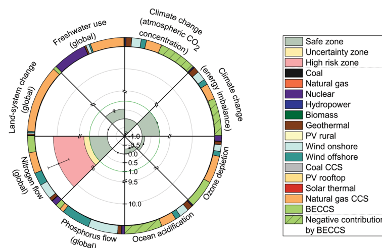
Fig. 4 Global US electricity generation and imports portfolio and performance relative to downscaled planetary boundaries for the planetary boundaries mix (solution S3). The circle on the left represents the energy mix in 2030 that would minimize the transgression of planetary boundaries at minimum cost; its performance in terms of planetary boundaries is shown in a rose chart on the right. The rose chart represents the current performance of each Earth-system process divided by the US power sector share of the full safe operating space (i.e., a value less than one implies it lies below the planetary boundary). The green zone is the safe operating space (i.e., within the strictest planetary boundary in the uncertainty range), the yellow zone is the uncertainty range of each planetary boundary and the red zone is beyond the least strict planetary boundary in the uncertainty range. Each error bar corresponds to one standard deviation considering the uncertainty in environmental burdens (i.e., life cycle inventory entries) connected to planetary boundaries. Each circular sector of the outer ring on the right represents the intensity of each technology on each planetary boundary. The labeling of solutions is given in Table 2.
