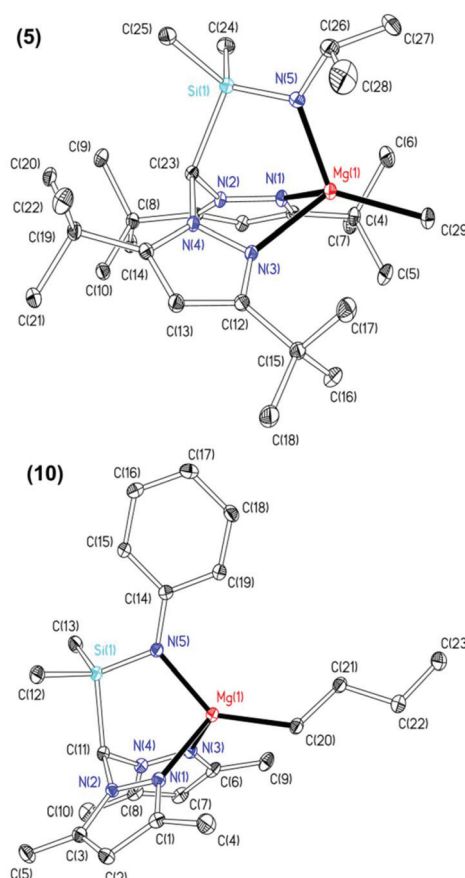
Fig. 1 Thermal displacement ellipsoid drawings (20% probability ellipsoids) of \text{Mg}\{\text{HC}(\text{tBu}_2\text{pz})_2\text{SiMe}_2\text{N}^t\text{Bu}\}\text{Me} ( 5 , top) and \text{Mg}\{\text{HC}(\text{Me}_2\text{pz})_2\text{SiMe}_2\text{NPh}\}^n\text{Bu} ( 10 , bottom). All hydrogen atoms have been omitted for clarity.
