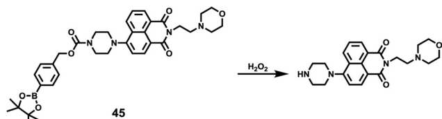
Scheme 34 Fluorescent probe 45 for H_2O_2 .
