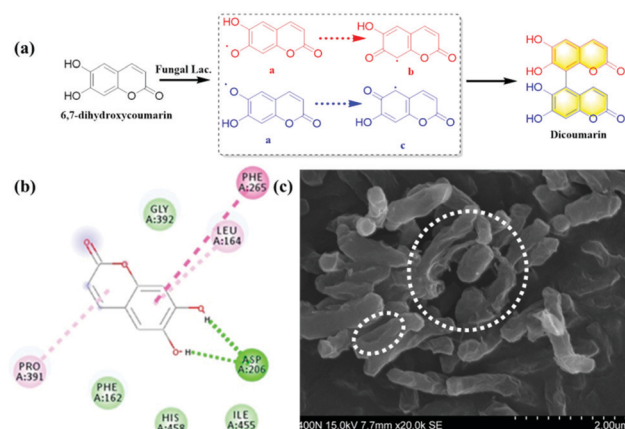
Fig. 5 The biosynthesis of dicoumarin mediated by fungal laccase and its inhibitory effect on Mycobacterium tuberculosis H37Ra. (a) The biosynthesis of dicoumarin from 6,7-dihydroxycoumarin mediated by fungal laccase. (b) In silico docking analysis between 6,7-dihydroxycoumarin and laccase. (c) The inhibitory effect of dicoumarin on Mycobacterium tuberculosis H37Ra measured by scanning electron microscope (SEM).
