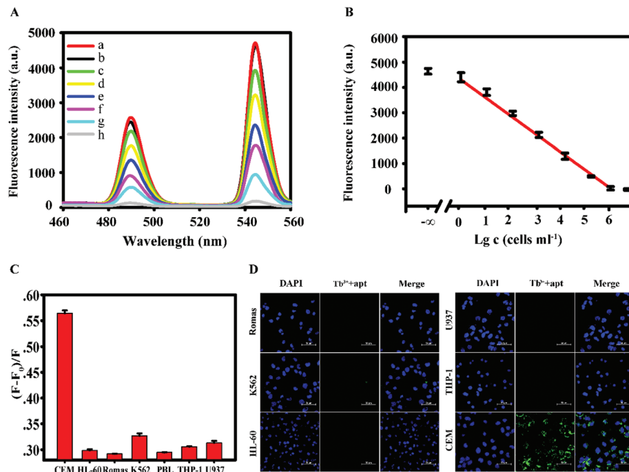
Fig. 3 (A) Fluorescence emission spectra of the Tb 3+ -apt fluorescent aptasensor in the presence of different concentrations of CCRF-CEM cells (a. Tb 3+ -apt, b. 10 0 cells per 200 \mu l, c. 10 1 cells per 200 \mu l, d. 10 2 cells per 200 \mu l, e. 10 3 cells per 200 \mu l, f. 10 4 cells per 200 \mu l, g. 10 5 cells per 200 \mu l, h. 10 6 cells per 200 \mu l). (B) Linear relationship between the fluorescence intensity and the concentration of CCRF-CEM cells. (C) Specificity of the fluorescent aptasensor for CEM. The fluorescence intensity rate (F - F_0)/F of the Tb 3+ -apt fluorescent aptasensor in the presence of CEM, HL-60, Ramos, K562, PBL, THP-1, and U937 cells, respectively ( 1 \times 10^6 cells per 200 \mu l), where F and F_0 are the fluorescence intensity without and with detection cells at 545 nm. Excitation: 290 nm. (D) Fluorescence micrographs of six different cells after mixing with Tb 3+ -apt. Nuclei were stained with DAPI. Scale bars indicate 50 \mu m.
