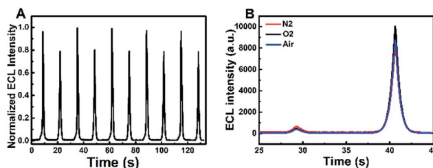
Fig. 2 (A) Continuous ECL responses of the GQDs– \text{K}_2\text{S}_2\text{O}_8\text{-Na}_2\text{SO}_3 system during a continuous potential scan between –1.2 and 1.5 V at a scan rate of 0.2 \text{V s}^{-1} (B) ECL-time profiles of the GQDs– \text{K}_2\text{S}_2\text{O}_8\text{-Na}_2\text{SO}_3 system in air-saturated (blue curve), nitrogen-saturated (red curve) and oxygen-saturated (black curve) 0.1 M PBS (pH 7.4) (scan potential: –1.2 to 1.0 V).
