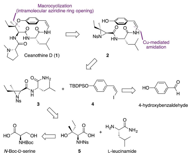
Scheme 1 Retrosynthetic analysis.
