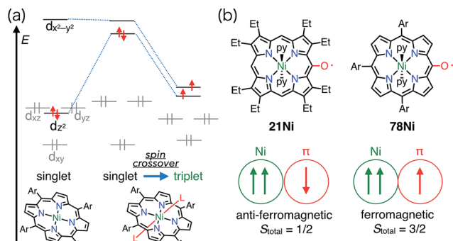
Fig. 25 (a) Coordination-induced spin crossover of Ni(II) center. (b) OEP and 10,15,20-triarylporphyrin meso -oxy radicals and their magnetic interaction with the Ni(II) center. Ar = pentafluorophenyl.
