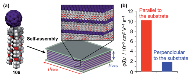
Fig. 17 (a) Schematic structure of an oriented 2D assembly of C_{60} units achieved by a tripodal triptycene-based 2D supramolecular scaffold ( 106 ) and (b) its maximum transient conductivities ( \phi \sum \mu ) sandwiched between quartz substrates along directions parallel (red) and perpendicular (blue) to the substrate as determined by flash-photolysis time-resolved microwave conductivity measurements.
