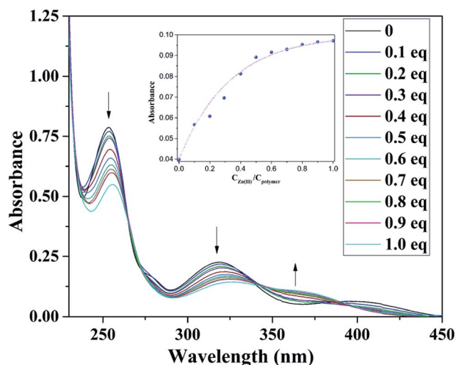
Fig. 2 Absorption spectra of 10 \text{ mol L}^{-1} copolymer with the addition of 0\text{--}15 \text{ mol L}^{-1} \text{ Zn}^{2+} . Inset: The absorbance ratio ( A_{383}/A_{346} ) as a function of \text{Zn}^{2+} concentration.
