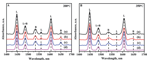
Fig. 9 FTIR spectra of pyridine adsorbed on different catalysts after degassing at (A) 200 °C and (B) 350 °C: (a) NiMo/Zr-in-F, (b) NiMo/Zr-gra-F, (c) NiMo/Zr-im-F.
