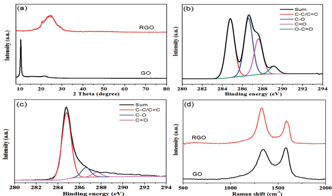
Fig. 2 (a) XRD patterns of GO and RGO; (b) C1s XPS spectrum of GO; (c) C1s XPS spectrum of RGO; (d) Raman spectra of GO and RGO.
