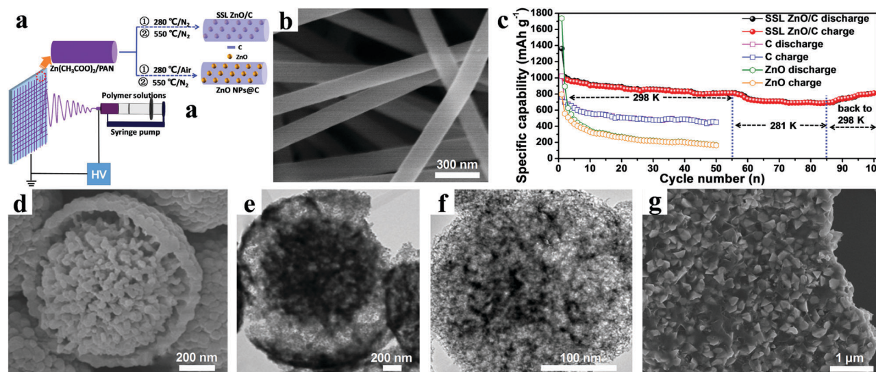
Fig. 9 (a) Schematic illustration of preparation process of SSL ZnO/C and ZnO NPs@C composites; (b) SEM image of SSL ZnO/C NFs; (c) cycling performance of SSL ZnO/C NFs at 0.1\text{ A g}^{-1} under the various ambient temperatures. Reproduced with permission. 98 Copyright 2015, Elsevier. (d) SEM image and (e) TEM image of yolk-shell structured YC-ZnO. Reproduced with permission. 100 Copyright 2017, Elsevier. (f) TEM image of a single ZnO-NMPCS particle. Reproduced with permission. 103 Copyright 2016, Elsevier. (g) SEM image of ZnO@C-5. Reproduced with permission. 105 Copyright 2014, Elsevier.
