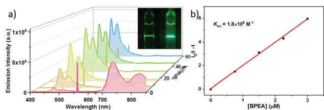
Fig. 2 (a) Luminescence spectra of Lu-1 with BPEA at different concentrations. Inset presents the photographs of BPEA (left) and Lu-1 /BPEA (right) solution irradiated with a 561 nm laser. (b) Stern–Volmer plot of Lu-1 with BPEA ( [\text{Lu-1}] = 0.5 \mu\text{M} , \lambda_{\text{ex}} = 561 \text{ nm} , 480 \text{ mW cm}^{-2} , in degassed toluene at room temperature).
