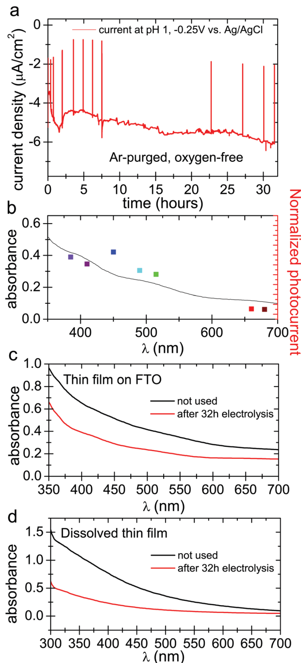
Fig. 4 Photocathodic experiments in oxygen-free electrolyte. (a) Chronoamperometry with solar simulator illumination over 32 hours at -0.25\text{V} vs. Ag/AgCl and deoxygenated pH 1 electrolyte. The positive spikes in the current trace are turning off of the light source in order to see the level of dark current in the sample. (b) Photocurrent action spectrum overlaid with the absorption spectrum of eumelanin on FTO for deoxygenated photocurrent. (c) Direct UV-VIS comparison between DHI eumelanin thin film used as a blank (150 nm) vs. DHI eumelanin thin film used in the 32 hour photo(electro)catalytic experiment (150 nm) and (d) UV-VIS comparison between dissolved eumelanin thin film used as a blank vs. dissolved eumelanin thin film used in the same experiment.
