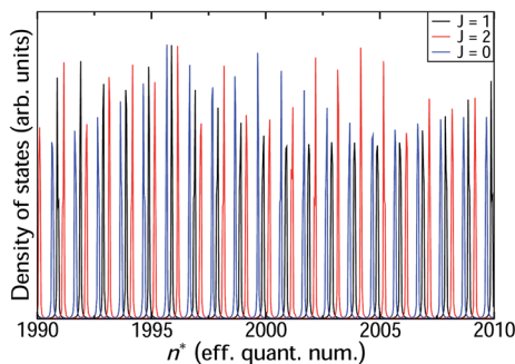
Fig. 6 Progression of heavy Rydberg resonances around the principal quantum number n = 2000 for J = 0, 1 and 2 . These states have classical turning points at around R_{tp} = 8700 \text{ a.u.}
